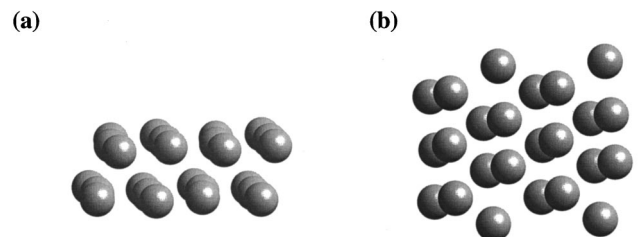
FIG. 2. Illustration of the Iodine sublattice at ambient pressure as viewed parallel (a) and perpendicular (b) to the double layers. It shows the highly symmetric arrangement of the atoms
