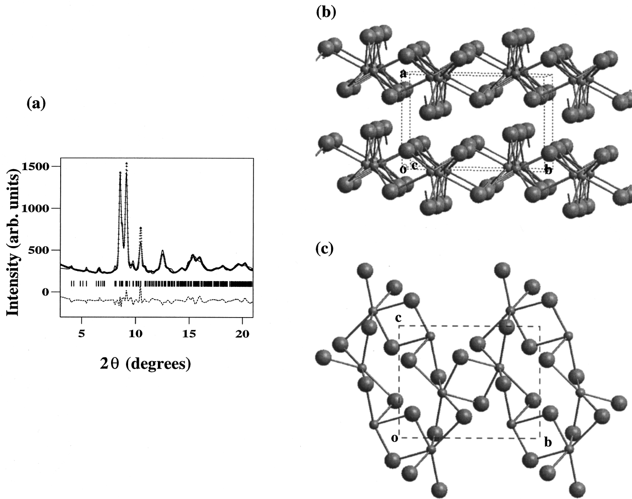
FIG. 7. Rietveld refinement of powder pattern of \text{SbI}_3 observed at 101 kbar (a). The fit shown in (a) has been obtained using a (100) preferred orientation correction. The reliability factor R_{wp}(\%) is 6.48. Illustration of the relevant pucker layered structure [having space group C_{2h}^5(P2_1/c) ] along different view point is shown in (b) and (c). The small and large spheres stand for the Sb atoms and I atoms, respectively.
