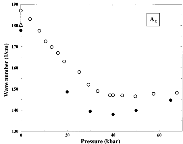
FIG. 12. The pressure variation of the X-I symmetric stretch vibrational mode for \text{AsI}_3 as obtained from Raman spectroscopic data (open circles) and from density functional calculations (filled circles) using full structural relaxation. The open triangle corresponds to the 12 K measurement at ambient pressure.
