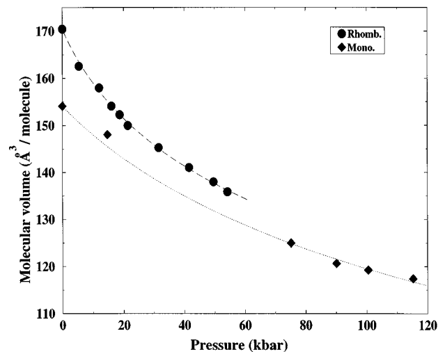
FIG. 9. Molecular volume vs pressure for \text{SbI}_3 illustrating the relatively small volume collapse and the irreversibility of the transition under decompression. The low-pressure phase (rhombohedral) is denoted as the solid circle whereas the high-pressure phase (monoclinic) is shown as the solid diamond. The dashed and dotted lines represent a fit to the Birch-Murnaghan equation of state.
