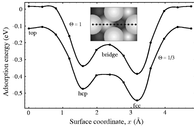
FIG. 4. The adsorption energy along a path connecting two top sites in the \langle 110 \rangle direction (see the inset figure) for the coverages \Theta = 1 and \Theta = \frac{1}{3} . The z coordinate is constrained to be the equilibrium distance from the surface, z_{eq} .
