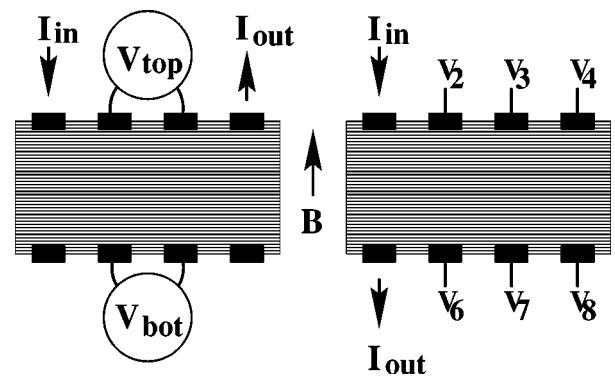
FIG. 1. The modified flux-transformer set-up of Safar et al. (Ref. 3). The diagram on the left shows the arrangement of the terminals for the top geometry, and the right shows the side geometry. The samples are single crystals of YBCO with the magnetic field aligned along the \hat{c} -axis of the crystal. V_{\text{left}} = V_2 - V_6 and V_{\text{right}} = V_3 - V_7 .
