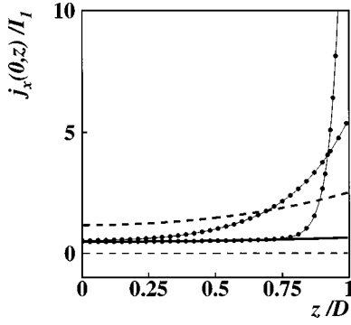
FIG. 9. The current density j_x(0,z) for different values of \ell corresponding to nontranslationally invariant conductivities of the form given by Eq. (34) with the same parameters and input current as in Fig. 8. The upper dashed curve is the local curve ( \ell \rightarrow \infty ), and the curves with closed circles are for \ell=0.4 and \ell=0.067 . The lower solid curve is the Huse and Majumdar result [ j_x(0,z) \approx 0.48 \cosh(0.815z) for the parameters used here], which corresponds to the \ell \rightarrow 0 limit of our results.
