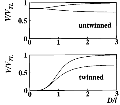
FIG. 6. The results for V_{top} and V_{bot} as a function of \ell , using the conductivities of Eq. (14) with parameters \sigma_x^{(n)} = 5 , \sigma_z^{(n)} = 1 , D = 1 , C_1 = 1 , and C_2 = 5 . The upper curve in each plot is V_{top} , and the lower is V_{bot} .
