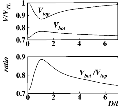
FIG. 4. The voltages V_{top} and V_{bot} and their ratio for the conductivity \hat{\sigma}_{zz}(k_x) = \sigma_z^{(n)} + C\ell e^{-k_x^2\ell^2/2} , with the same values of parameters as in Fig. 3. By definition, V_{TL} is defined to be V_{top} in the local case for this geometry, which can be calculated from Eq. (A2). Note that V_{bot}/V_{top} does not tend to 1 as \ell \rightarrow \infty .
