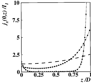
FIG. 8. The current density j_x(0,z) for different values of \ell corresponding to the case (2) Padé conductivities, Eqs. (15b) and (28), with parameters: \sigma_x^0=5 , \eta=5 , \Sigma_z=1 , D=1 , L=5 and input current I(x)=I_1\sin(\pi x/L) . The dashed curve is the local curve ( \ell \rightarrow \infty ), and the other curves are for \ell=0.4 , and \ell=0.067 . The areas under the curves are equal, but as \ell becomes smaller there is more current density at the surface.
