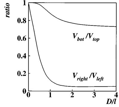
FIG. 3. The ratios of V_{\text{bot}}/V_{\text{top}} and V_{\text{right}}/V_{\text{left}} for the conductivity with positive viscosity coefficients, the form of which is provided in the text. The boundary conditions used were J_T(x) = J_0[\delta(x-2L_c) - \delta(x+2L_c)] and J_S(x) = -J_0 \delta(x+2L_c) ( 4L_c is defined to be the distance between the current inputs). The voltages V_{\text{top}} and V_{\text{bot}} were measured at x = \pm L_c as were the voltages V_2, V_3, V_6, and V_7 . The parameters used are \Sigma_x = 5 , \sigma_z^{(n)} = 1 , C = 1 , D = 1 , and L_c = 1 ; this corresponds to measuring lengths in terms of the thickness of the sample and conductivities in terms of \sigma_z^{(n)} , as will also be done in all the other figures.
