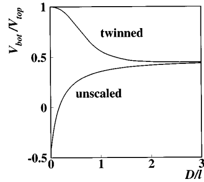
FIG. 7. The results obtained for the ratio V_{\text{bot}}/V_{\text{top}} for case (2). The conductivities used are given by Eq. (15b) for the lower curve, and Eq. (C3b) for the upper curve (which has the appropriate scaling for a twinned sample). The parameters used are \Sigma_x = \sigma_x^{(n)} = 5 , \Sigma_z = \sigma_z^{(n)} = 1 , \ell_{\parallel} \equiv \ell , D=1 , L=5 , C_1=1 , C_2=5 , and \Delta_x^z = 5\ell^2 —note the scaling with \ell which is present. For the twinned case, V_{\text{bot}}/V_{\text{top}} does in fact tend to 1 as \ell \rightarrow \infty .
