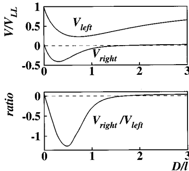
FIG. 5. The voltages V_{left} and V_{right} and their ratio for the conductivity \hat{\sigma}_{zz}(k_x) = \sigma_z^{(n)} + C\ell e^{-k_x^2\ell^2/2} , with the same parameters as for Figs. 3 and 4. Here, V_{LL} is defined to be V_{left} for the local case, Eq. (A2). The notable feature here is that V_{right} becomes negative.
