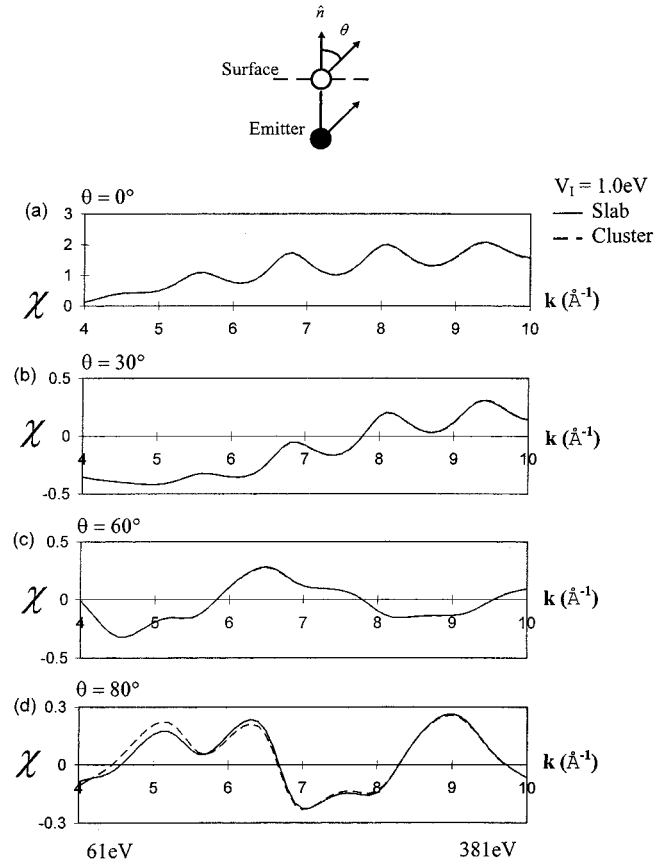
FIG. 13. Same as in Fig. 11, except V_0=0 eV and V_I=1.0 eV are used.
