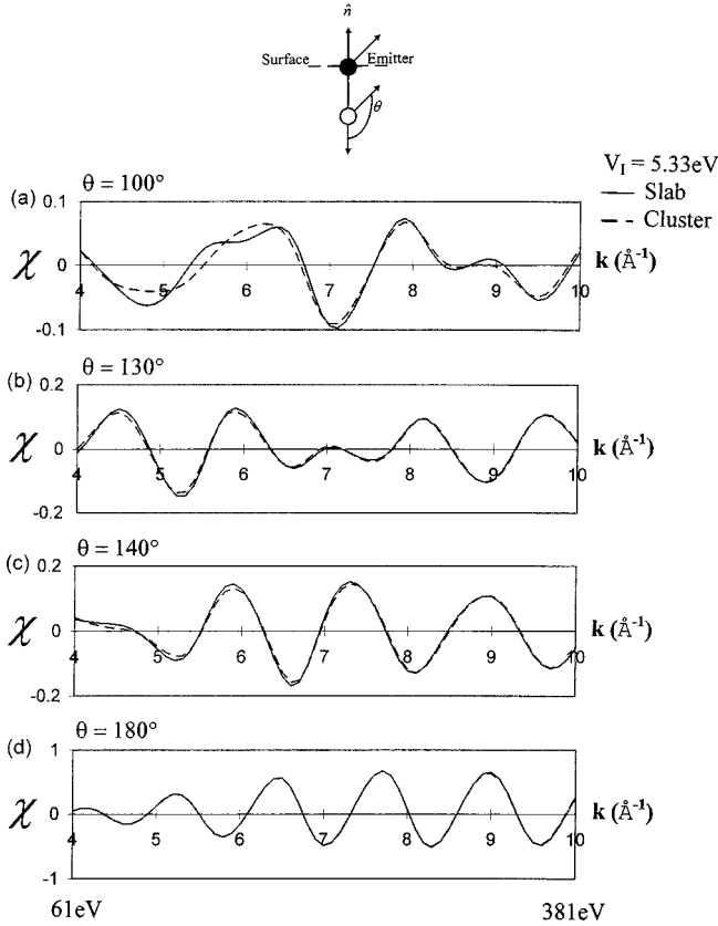
FIG. 12. Same as in Fig. 11, except for various backscattering angles.
