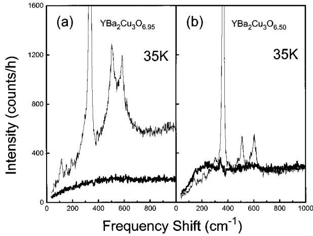
FIG. 3. A comparison of the Raman spectra of Y123 measured in the B_{1g} (thin lines) and B_{2g} (bold lines) geometries of (a) optically doped and (b) underdoped samples.
