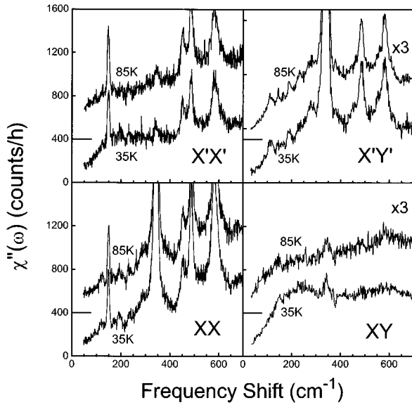
FIG. 1. The Raman response functions ( \chi'' ) of \text{YBa}_2\text{Cu}_3\text{O}_{6.5} obtained at 85 K and 35 K in the X'X' ( A_{1g} + B_{2g} ), X'Y' ( B_{1g} ), XX ( A_{1g} + B_{1g} ), and XY ( B_{2g} ) scattering geometries, which are obtained by dividing the original spectra by the Bose-Einstein thermal factor. The XY and X'Y' spectra have been scaled by a factor of 3 to place them on the indicated scale. The 85 K spectra have been displaced upward and the zero level is indicated by the horizontal bar at the left.
