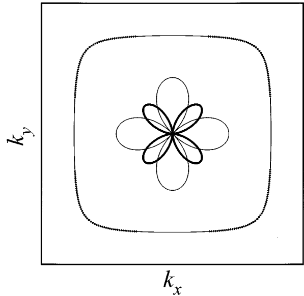
FIG. 2. Schematic illustration of the FS for optimally doped Y123 (solid thin line) and polar plots (see Ref. 28) showing the k dependence of the magnitude of the X'Y' ( B_{1g} ) (thin solid line) and XY ( B_{2g} ) (thick solid line) components of the Raman tensor (1). For a calculation of the spectra in the underdoped compounds (see Fig. 4) it will be assumed that spectral weight is present only on the dashed portions of the FS.
