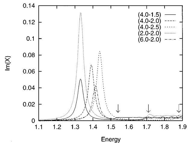
FIG. 4. The influence of Coulombic parameters, U_0 and V_0 , on \text{Im}\chi(\omega) in the absence of pumping. The value of (U_0 - V_0) is indicated for each curve. The arrows (from left to right) indicate the band edges for the curves (4-1.5), (4-2.0), and (4-2.5), respectively. Their positions shift linearly with V_0 . On the contrary, the band edge is not affected by varying U_0 (cannot be seen easily from the figure). The energy is in units of 4 \delta t .
