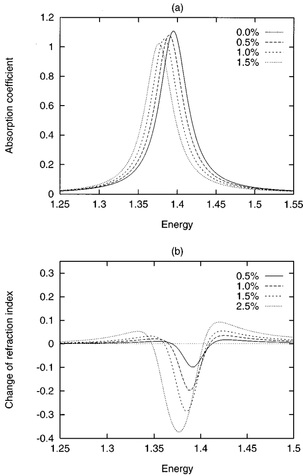
FIG. 2. The effect of different exciton concentrations on (a) absorption coefficient \alpha and (b) the change of refraction index \delta n . \alpha is in units of 2.0 \times 10^4 \text{ cm}^{-1} . The energy is in units of 4 \delta t .
