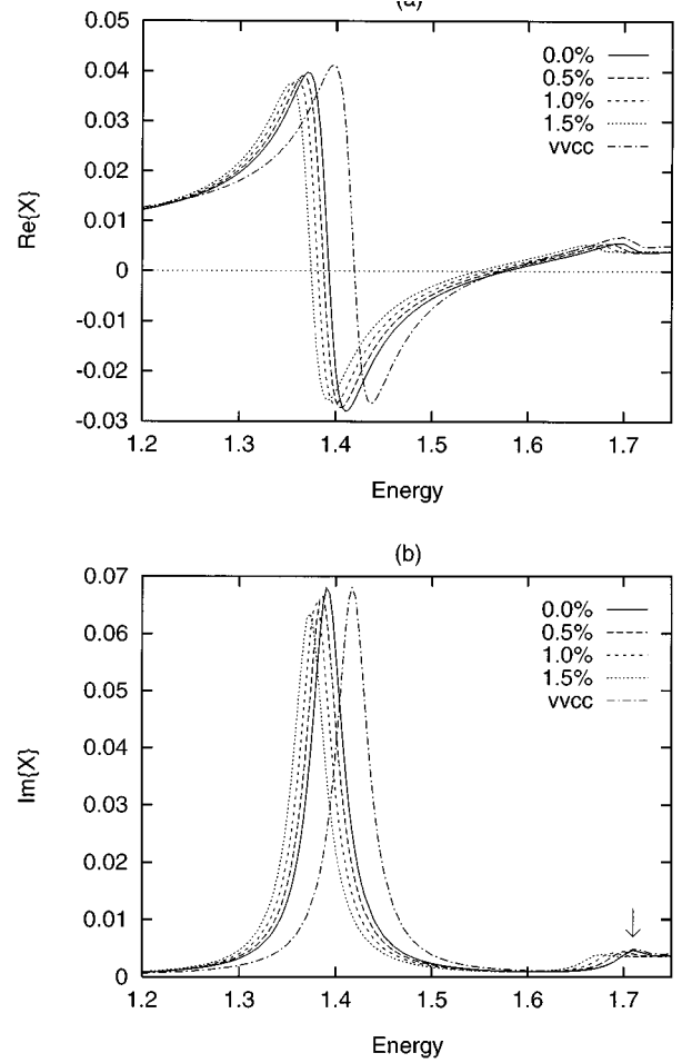
FIG. 1. Real (a) and imaginary (b) parts of \chi(\omega) for different exciton concentrations, labeled by the percentages of the occupation of conduction band (0, 0.5%, 1.0%, and 1.5%) at room temperature. Probe energy is in units of the bare band gap, 4\delta t . The ‘‘vvc’’ curve comes from the calculation without the \mathcal{V}_{vvc}^{kk'} and \tilde{\mathcal{V}}_{vvc}^{kk'} terms and in the absence of excitons. The arrow at the bottom right of Fig. 1(b) indicates the position of the band edge for the solid line.
