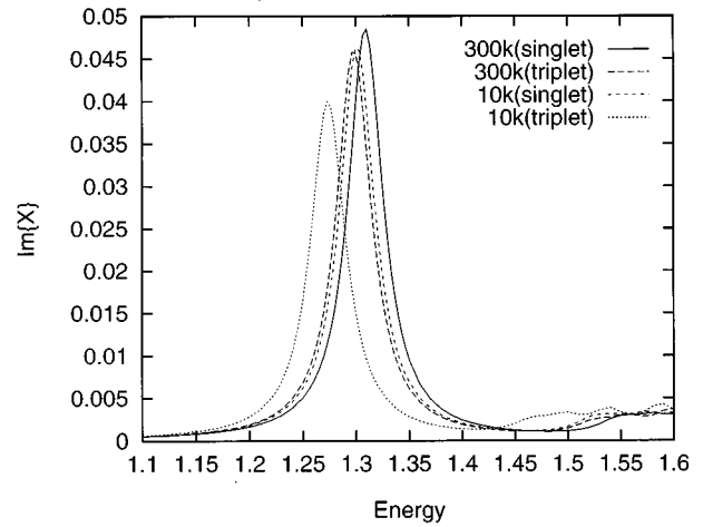
FIG. 3. The effect of temperatures and singlet/triplet populations on \text{Im}\chi(\omega) . The percentage of conduction electrons is 2.5% for all of the curves. At room temperature, it makes small difference whether the excitons are singlet or triplet. The distinction is more apparent at 10 K.
