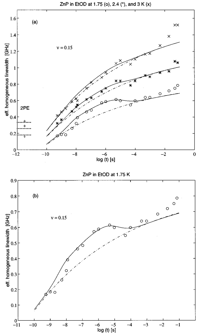
FIG. 2. (a) 3PE decay rates, [1/\pi T_2^*](t) , as a function of the waiting time t for ZnP in EtOD, from Ref. 15. The lines are fits to the data: (—) heating effects included [Eq. (26)], (---) no heating effects included [Eq. (19)]. Effective relaxation rates used are R_{\text{eff}} = 1.2 \times 10^9 \text{ s}^{-1} ( \circ ), R_{\text{eff}} = 2.8 \times 10^9 \text{ s}^{-1} ( * ), R_{\text{eff}} = 3.5 \times 10^9 \text{ s}^{-1} ( \times ). The parameters for the heating process are \tau_a = 15 \mu\text{s} , T_1 = 2.65 \text{ K} ( \circ ), T_1 = 2.8 \text{ K} ( * ), and T_1 = 3.3 \text{ K} ( \times ). The values of the 2PE decay rates are also given in the figure (+) along with the prediction of the model (dotted lines) with K_p = 26.9 \text{ MHz/K}^{1+\nu} . The contribution of \Gamma_{\text{PLM}} is neglected in the fits at all three temperatures. (b) Same as (a) but only the data at T_0 = 1.75 \text{ K} are shown.
