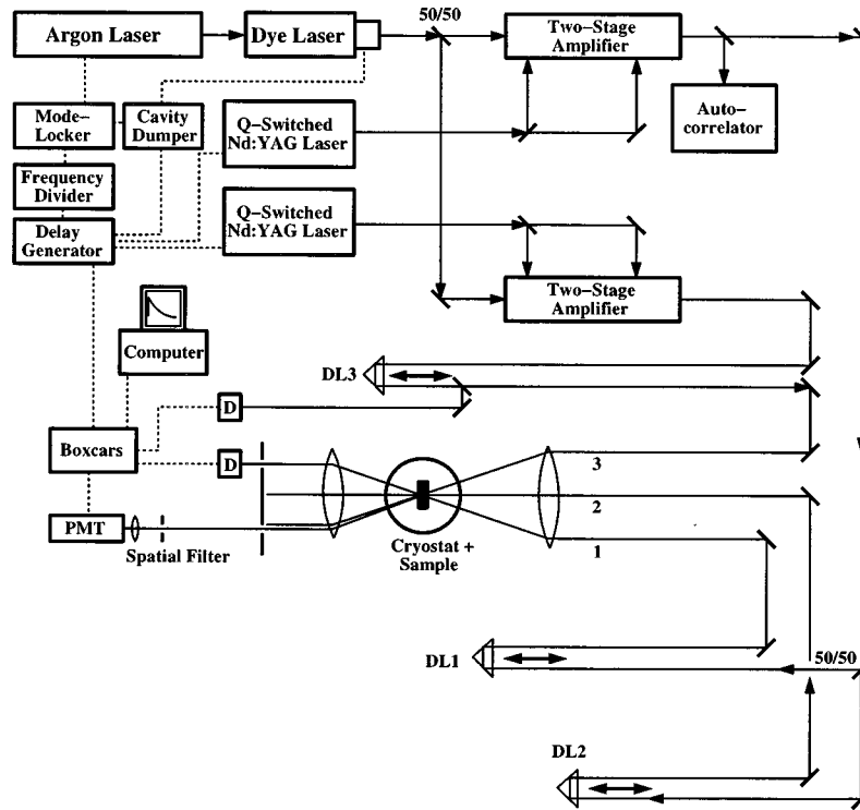
FIG. 1. Experimental setup for stimulated photon echo measurements. “50/50” marks 50% beam splitters, DL1-3 are optical delay lines, D photodiodes, and PMT is a photomultiplier tube.
