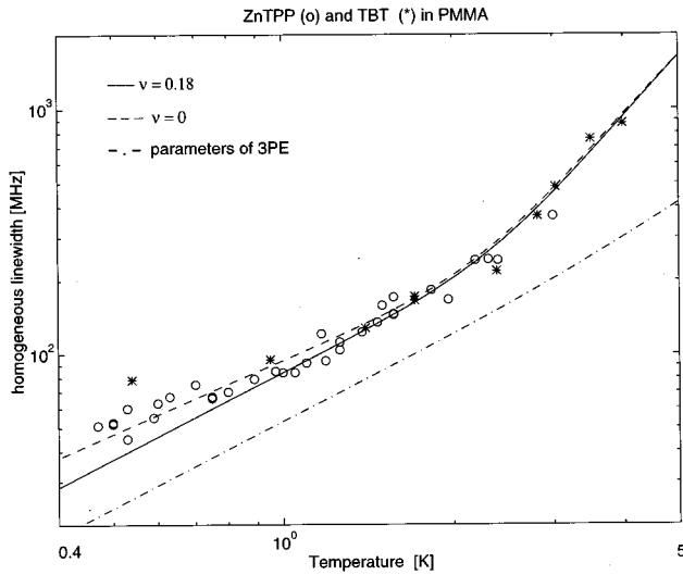
FIG. 4. 2PE decay rate, [1/\pi T_2^*]_{2PE} , for ZnTPP ( \circ ) and TBT ( * ) in PMMA. The solid line is a fit of Eq. (28) to the data for \nu = 0.18 , K_\nu = 24 MHz/K ^{1+\nu} , b = 15.8 GHz, and \Delta E = 9.7 cm ^{-1} . The dashed line is a fit of Eq. (28) with \nu = 0 , K = 25.7 MHz/K, b = 12.7 GHz, and \Delta E = 8.8 cm ^{-1} . The dashed dotted line shows Eq. (28) with parameter values obtained from the fit to the 3PE data [Fig. 2(a)]: \nu = 0.18 , K_\nu = 15.2 MHz/K ^{1+\nu} , b = 0.9 GHz, and \Delta E = 9.7 cm ^{-1} .
