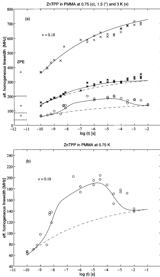
FIG. 3. (a) 3PE decay rates, [1/\pi T_2^*](t) , as a function of the waiting time t for ZnTPP in PMMA, from Ref. 18. The lines are fits to the data: (—) heating effects included [Eq. (26)], (---) no heating effects included [Eq. (19)]. Effective relaxation rates used are R_{\text{eff}} = 10^{11} \text{ s}^{-1} ( \circ ), R_{\text{eff}} = 1.3 \times 10^{11} \text{ s}^{-1} ( * ), R_{\text{eff}} = 2.6 \times 10^{11} \text{ s}^{-1} ( \times ). The parameters for the heating process are \tau_a = 300 \mu\text{s} , T_1 = 1.5 \text{ K} ( \circ ), T_1 = 1.7 \text{ K} ( * ), and T_1 = T_0 ( \times ). The values of the 2PE decay rates are also given in the figure (+) along with the prediction of the model (dotted lines) with K_\nu = 15.2 \text{ MHz/K}^{1+\nu} , b = 0.9 \text{ GHz} , and \Delta E = 9.7 \text{ cm}^{-1} . (b) Same as (a) but only the data at T_0 = 0.75 \text{ K} are shown.
