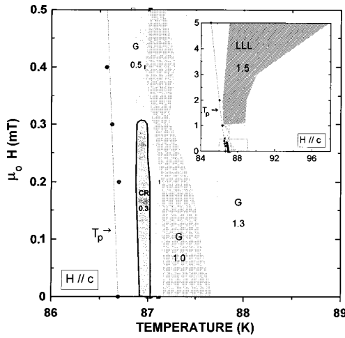
FIG. 4. H - T diagram showing the regions of dominance of Gaussian and critical scaling in the low-field limit of the H||c configuration. The regions are labeled by the observed exponents. The location of the 3D-XY regime is marked by a contour. The inset shows the large domain at higher fields where the LLL scaling is observed. The area limited by the dotted lines is enlarged in the main picture.
