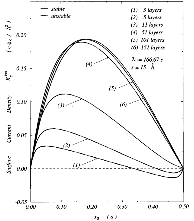
FIG. 3. Plots of the bottom layer surface current density K_y^{\text{bot}} versus the bottom lattice displacement x_0 for 3, 5, 11, 51, 101, and 151 layers. A 0.1 T magnetic field is applied perpendicular to the layers, such that a = 103.02s .
