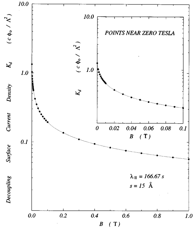
FIG. 5. Semilog plots for the magnetic field dependence of the decoupling surface current density K_d (applied in opposite directions to the top and bottom layers) needed to magnetically decouple the outermost 2D pancake lattices from those in the interior. The number of layers is 101. The value of K_d in the zero-field limit is included.
