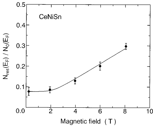
FIG. 3. Magnetic field dependence of the DOS fraction, N_{\text{res}}(E_F)/N_0(E_F) . The solid line indicates the calculation based on the simple model that the V-shaped DOS is split by the magnetic field as illustrated in Fig. 1(b).
