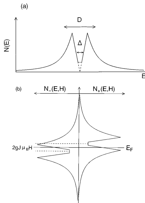
FIG. 1. (a) Schematic density of states (DOS) with the V-shaped pseudogap. Bandwidth, D=140 K, magnitude of gap, \Delta=14 K, and N_{\text{res}}/N_0=0.077 were obtained in the previous work (Ref. 5). (b) Schematic DOS split by magnetic field. N_+(E,H) and N_-(E,H) are the DOS of up- and down-spin bands, respectively.
