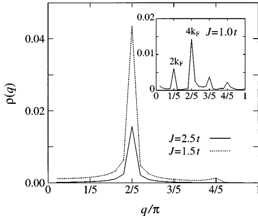
FIG. 2. Fourier components of the charge density oscillations. The system size is 60 sites and the carrier density is n_c=4/5 . The solid line and the broken line correspond to J=2.5t and J=1.5t , respectively. The Fourier transformation is carried out by using the central 50 sites. The inset shows the result for J=1.0t , for which typical truncation errors are 4 \times 10^{-5} .
