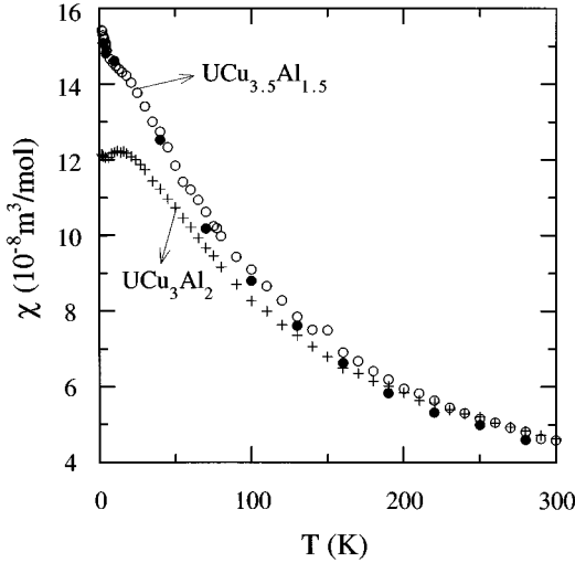
FIG. 4. Temperature dependence of the magnetic susceptibility of polycrystalline \text{UCu}_{3.5}\text{Al}_{1.5} ( \circ ) and \text{UCu}_3\text{Al}_2 ( + ). The solid circles represent the M/H values of \text{UCu}_{3.5}\text{Al}_{1.5} in an applied field of 18 T.
