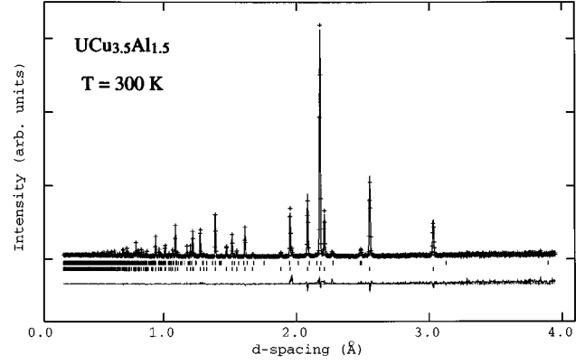
FIG. 9. Observed and calculated nuclear structure profile of \text{UCu}_{3.5}\text{Al}_{1.5} at 300 K, as measured on the +90^\circ bank of NPD. Starting from the bottom, the reflection markers denote \text{UCu}_{3.5}\text{Al}_{1.5} (with parameters as given in Table I) and \text{U}_2\text{Cu}_9\text{Al} . The difference of measured and calculated intensities is shown by the solid line below. The intensities have been divided by the incident spectrum.
