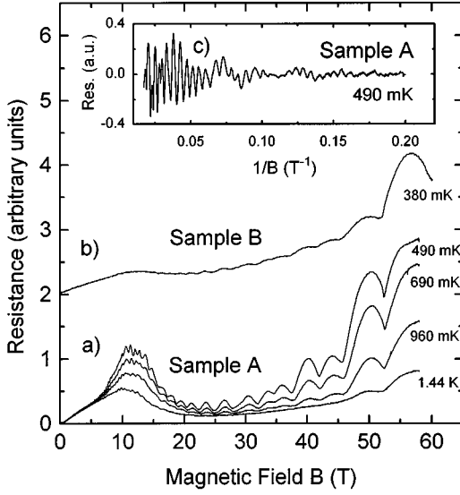
FIG. 2. (a) Magnetoresistance of sample A of \beta' -(BEDT-TTF) 2 AuBr 2 for temperatures in the range 490 mK to 1.44 K. (b) Magnetoresistance of sample B of \beta' -(BEDT-TTF) 2 AuBr 2 at 380 mK. (c) Oscillatory component of the 490 mK trace of (a) derived using division by an exponential polynomial approximation to the classical background magnetoresistance.
