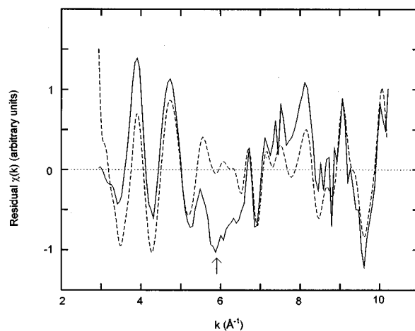
FIG. 1. Residual function after a first shell model fit is subtracted from the raw experimental metaphosphate glass data; before (solid line) and after (dashed line) Fourier filtering to remove the anomalous feature at \sim 6 \text{ \AA}^{-1} (marked by the arrow) which is most likely an artifact of a double-electron excitation event.
