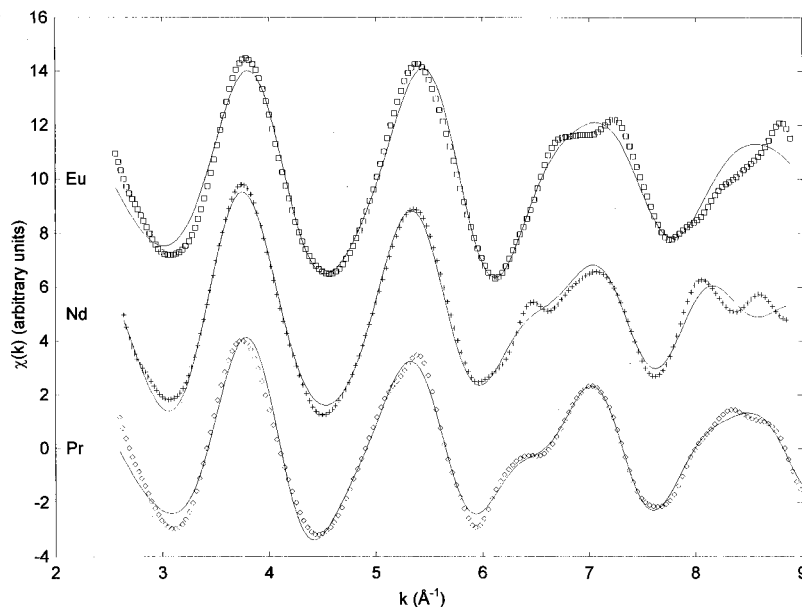
FIG. 3. Praseodymium, neodymium, and europium metaphosphate glass EXAFS \chi''(\mathbf{k}) , experimental data (points) and theoretical fits (lines).
