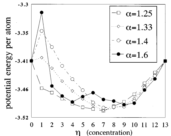
FIG. 4. The lowest minimum in the spectra plotted as a function of the concentration for the four values of \alpha . The energy is in LJ units. The three lower values of \alpha have a similar parabolic shape with the same minimum at \eta=7 and all the minima have an icosahedral cage, while the 1.6 case has a double-well shape and the icosahedral structures are limited only for \eta > 7 .
