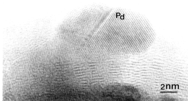
FIG. 2. High-resolution transmission electron microscopy picture showing a Pd nanocrystal in the upper right corner. An internal twin boundary is visible in the nanocrystal.
