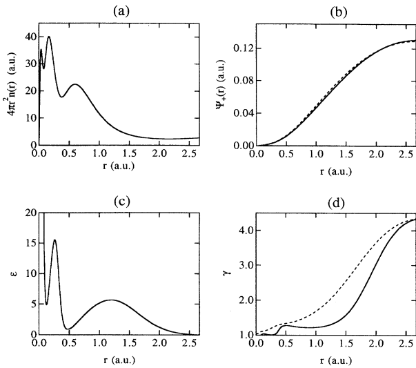
FIG. 1. (a) Spherically averaged radial electron density within the Wigner-Seitz sphere in Cu. (b) The corresponding positron wave function, (c) parameter \epsilon [Eq. (3)], and (d) the enhancement factor in the LDA (dashed line) and in the GGA (solid line).
