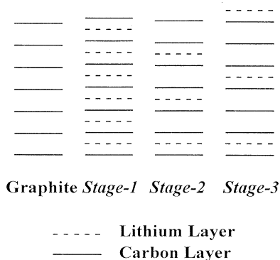
FIG. 1. Schematic diagram of the staged phases of Li intercalated graphite.
