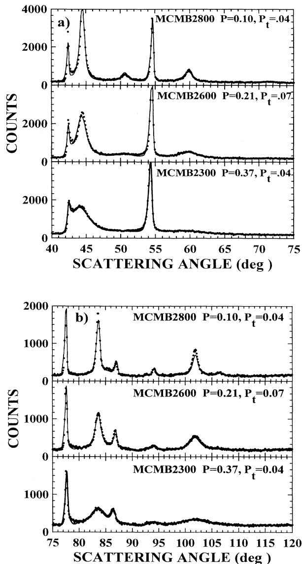
FIG. 3. The x-ray-diffraction patterns (points) and calculated best fits from the structure refinement program (solid lines) for the samples MCMB 2800, 2600, and 2300. (a) 40^\circ \leq scattering angle \leq 75^\circ . (b) 75^\circ \leq scattering angle \leq 120^\circ .
