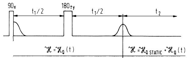
FIG. 1. 2D NMR pulse sequence for elimination of the static part of the quadrupole interaction from the \omega_1 domain, while retaining the dynamic part. The sequence is designed for half-integer spins I > \frac{1}{2} with only the central transition \frac{1}{2} \rightarrow -\frac{1}{2} irradiated. Since only two levels are involved the problem is formally equivalent to the separation of chemical shift from dipole coupling for spins I = \frac{1}{2} . In the \omega_2 domain the static line shape convoluted with the dynamic one is obtained, reflecting the full Hamiltonian \mathcal{H}_{Q\text{static}} + \mathcal{H}_Q(t) . In the \omega_1 domain, only the dynamic line shape appears, reflecting the dynamic part of the quadrupole Hamiltonian \mathcal{H}_Q(t) .
