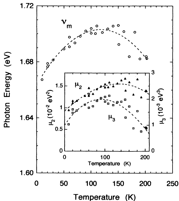
FIG. 3. Temperature dependence of \nu_m ( \circ ), \mu_2 ( \triangle ), and \mu_3 ( \square ) of the A band. Dashed lines are drawn as guides.
