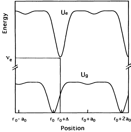
FIG. 4. A model of the ground- and excited-state potentials of the soliton as a function of the position in an MX chain. r_0 refers to an equilibrium position, a_0 to the nearest Pt-Pt distance in a chain, and \Delta to the relative displacement of the potential minima.
