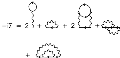
FIG. 1. Dyson equation for the self-energy of the Holstein model. The solid lines denote the bare (electronic) Green's function G_0 and the wavy lines denote the phonon propagator. The self-energy includes the Hartree and Fock contributions, the second-order dressing of the phonon line, the lowest-order vertex correction, and the second-order rainbow diagram (which arises from the self-energy insertion of the Fock diagram into the Fock diagram).
