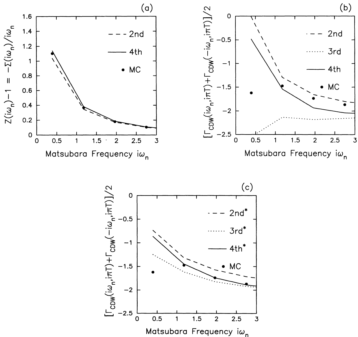
FIG. 11. Same as in Fig. 10, but with a stronger value of the coupling ( U = -2t^* , T = t^*/8 ). The self-energy is still reproduced accurately by all orders, but only the third-order IPT approximation has the correct qualitative behavior for the vertex.
