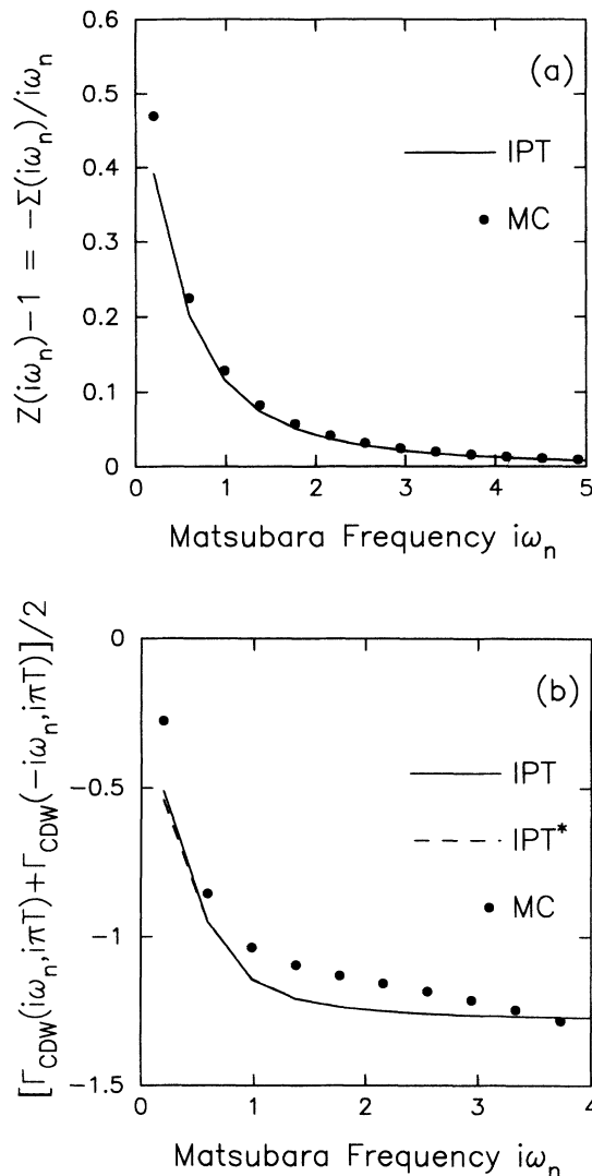
FIG. 3. Comparison of the second-order IPT (solid line) and IPT* (dashed line) to the QMC solutions (solid dots) for the Holstein model at half-filling with phonon frequency \Omega = 0.5t^* , interaction strength g = 0.4t^* , and temperature T = t^*/16 . This example is generic for the weak-coupling limit. In (a) the self-energy renormalization function Z(i\omega_n) - 1 is plotted against the Matsubara frequency. In (b) the symmetric combination of the first column of the irreducible vertex function in the CDW channel is shown. Note that even at this weak a value of coupling strength the third-order diagrams must play an important role.
