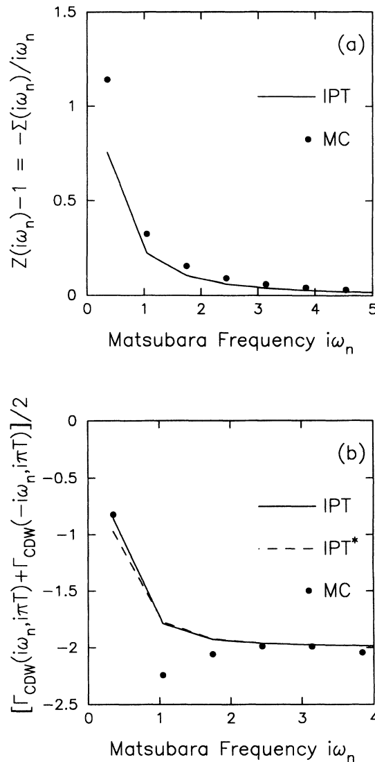
FIG. 4. Comparison of the second-order IPT (solid line) and IPT* (dashed line) to the QMC solutions (solid dots) for the Holstein model at half-filling with phonon frequency \Omega = 0.5t^* , interaction strength g = 0.5t^* , and temperature T = t^*/9 . This example is generic for the transition region to the strong-coupling limit. The self-energy renormalization function (a) and the irreducible vertex function in the CDW channel (b) are pictured. Note that in the limit where the strong-coupling effects begin to manifest themselves, the QMC vertex becomes increasingly attractive at low-frequency transfer.
