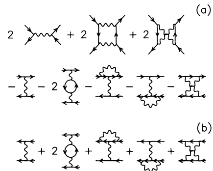
FIG. 2. The irreducible vertex functions in the CDW and SC channels. The CDW irreducible vertex function is shown in (a). Note that the vertex corrections (exchange diagrams) modify the interaction to lowest order in the CDW channel. The SC irreducible vertex function is shown in (b). The vertex corrections first enter at second order in the SC channel. In the IPT approximation the electron propagator is the bare Green's function G_0 , while in the IPT* approximation the electron propagator is the dressed Green's function G .
