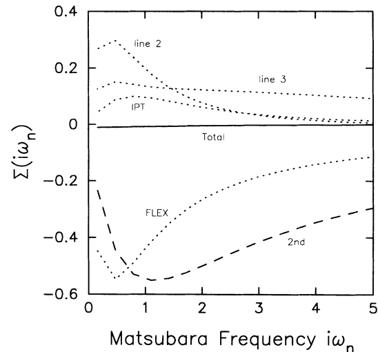
FIG. 9. Near cancellation of the fourth-order contributions to the self-energy. The second-order contribution to the self-energy (dashed line) is compared to each of the four fourth-order contributions (dotted lines) and the net fourth-order contribution (solid line) at U = -t^* , T = t^*/20 , and half-filling. The dotted line denoted FLEX corresponds to the first line of the fourth-order contributions in Fig. 8. The labels line 2 and line 3 denote the next two lines of fourth-order contributions in Fig. 8, and the label IPT refers to the last line in Fig. 8 corresponding to the second-order self-energy insertions into the second-order diagrams. Note that the total contribution of the fourth-order diagrams is an order of magnitude smaller than any of the individual classes of diagrams in Fig. 8, and that it is the same sign as the FLEX contributions.
