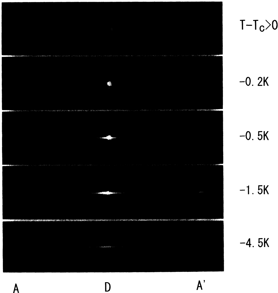
FIG. 1. Temperature dependence of the intensity distribution of transmitted and refracted light spots on the screen. The laser light was incident perpendicularly on the bc plane of KD_3(SeO_3)_2 crystal.
