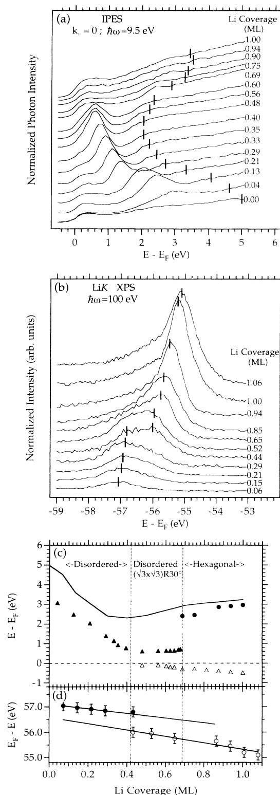
FIG. 2. (a) Normalized inverse-photoemission spectra for various coverages of Li on Be(0001). (b) Li 1s core-level spectra for various Li coverages on Be(0001). (c) Peak positions from inverse-photoemission and photoemission spectra as a function of coverage (symbols) and measured work function (solid line). The observed LEED patterns are indicated. (d) Measured 1s binding energy as a function of coverage. Lines are linear fits in each phase.
