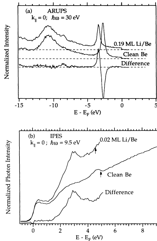
FIG. 1. Normalized photoemission (a) and inverse-photoemission (b) spectra for clean and Li-covered Be(0001). In (b), the arrows indicate the position of the vacuum level. The slight increase in emission evident in the difference spectra is understood as due to reduced momentum conservation in the presence of the disordered overlayer.
