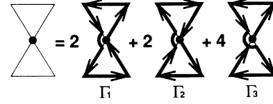
FIG. 2. An “hourglass” loop made of two triangles can be traversed in eight different ways, contributing three different phase factors to m_6 . On the right-hand side, there are three possible different paths: \Gamma_1 , \Gamma_2 , and \Gamma_3 . Path \Gamma_1 ( \Gamma_2 ) contributes e^{i\phi+i\phi} = e^{2i\phi} ( e^{-i\phi-i\phi} = e^{-2i\phi} ) to m_6 . In path \Gamma_3 the phases cancel and the contribution of this path to m_6 is e^{i\phi-i\phi} = 1 . The coefficients in front of the \Gamma 's are the number of paths with the same phase factor.
