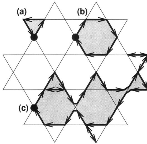
FIG. 1. Several examples of closed paths on a kagomé lattice and their respective phase factor contributions to the lattice path integrals. (a) Traversing counterclockwise a three-step path on an elementary triangular cell contributes a term e^{i\phi} to m_3 , (b) a six-step clockwise walk on an elementary hexagonal loop contributes a term e^{-6i\phi} to m_6 , and (c) a closed path of 26 steps with several links retraced. Its phase factor is e^{-16i\phi} . The solid dots denote the starting (and ending) sites and the arrows specify the hopping directions on bonds.
