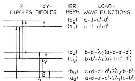
FIG. 2. Electron energy-level scheme of the divacancy as shown in Fig. 1, with LCAO wave functions and allowed electric dipole transitions indicated.
