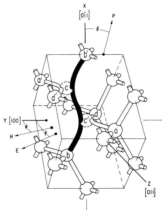
FIG. 1. Model of the divacancy, showing the crystallographic axes and the XYZ coordinate system of the defect. \vec{P} is the transition dipole moment. \vec{H} denotes the magnetic field direction as varied in the EPR experiments. \vec{E} is the direction of the electric field vector of the polarized light.
