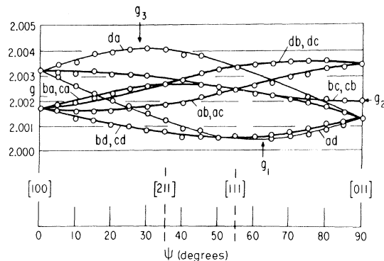
FIG. 4. G_6 EPR spectrum for the positively charged divacancy V_2^+ vs orientation of the magnetic field \vec{H} in the (0\bar{1}1) plane (from Ref. 3). The labels denote the defect orientation (see text).
