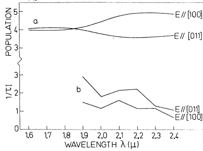
FIG. 5. (a) Saturation population and (b) alignment rate 1/\tau I ( \tau is the time constant, I the light intensity) vs wavelength \lambda for the incident light polarized along [100] or [011] for the group of divacancy orientations ad , da , bc , and cb , as monitored by the low-field resonance for \vec{H} \parallel [100] .
