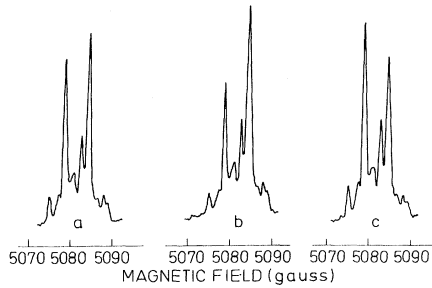
FIG. 3. EPR spectrum of the positively charged divacancy V_2^+ for \vec{H} \parallel [011] ; (a) the spectrum before illumination, (b) after illumination with polarized light, \vec{E} \parallel [100] , \lambda = 2.2 \mu , (c) after illumination with polarized light, \vec{E} \parallel [011] , \lambda = 2.2 \mu .
