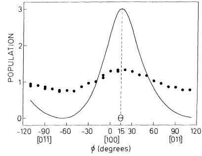
FIG. 8. Angular dependence of the number of divacancies in the orientation da . The solid line is calculated by the model for \theta = +15^\circ ; the dots represent the experimental behavior, \lambda = 2.15 \mu .
