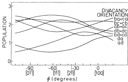
FIG. 6. Population of the various divacancy orientations after illumination with polarized light with \vec{E} in the (011) plane, for a wavelength \lambda = 2.15 \mu .
