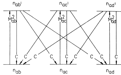
FIG. 7. Schematic of the model for reorientation within the Jahn-Teller triplet consisting of the divacancy orientations ab , ac , and ad .
