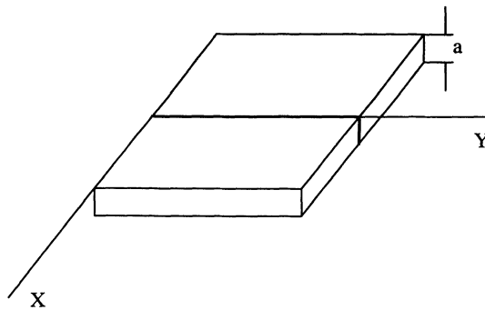
FIG. 1. A superconducting film with a Josephson junction (thick line).
