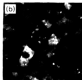
FIG. 6. (a) Evolution of 775-eV Co and 237-eV Pt Auger line intensities as a function of time at an annealing temperature of 750 K. The values are normalized to the measured pure bulk intensities. The interpolating line is a guide to the eye. (b) 400 \times 400 -nm 2 image of a 2-ML Co film after 30 min at 750 K.
