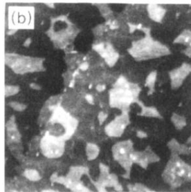
FIG. 6. (a) Evolution of 775-eV Co and 237-eV Pt Auger line intensities as a function of time at an annealing temperature of 750 K. The values are normalized to the measured pure bulk intensities. The interpolating line is a guide to the eye. (b) 400 \times 400\text{-nm}^2 image of a 2-ML Co film after 30 min at 750 K.
