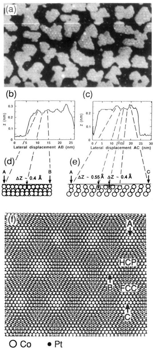
FIG. 4. 200 \times 120\text{-nm}^2 image of 1.6 ML of Co on Pt(111) showing Moiré fringes. (a) top view; (b) experimental trace (raw data) along same direction as AB in 4(f); (c) experimental trace (raw data) along same direction as AC in (f); (d) cross section along AB in (f); (e) cross section along AC in (f); and (f) top view of the hard-sphere model of the atomic arrangement of the Pt(111) substrate, the first, and a second 10% contracted Co layer.
