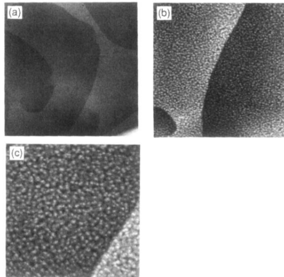
FIG. 3. Images of 2.8-ML Co on Pt(111) at a substrate region with a high density of screw dislocations. (a) 1000 \times 1000 \text{ nm}^2 , (b) 400 \times 400 \text{ nm}^2 , and (c) 200 \times 200 \text{ nm}^2 .
