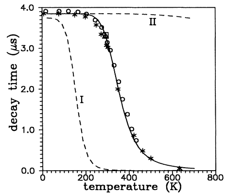
FIG. 3. Luminescence decay time for Ti:sapphire vs temperature. Dashed curves correspond to the sets of the input parameters of configuration-coordinate diagrams as follows: I corresponds to K_T = 0 , K_E = 0.289 , E_{\text{JT}}(E) = 2909 \text{ cm}^{-1} , E_{\text{JT}}(T) = 158 \text{ cm}^{-1} ( E_{\text{NR}} = 2633 \text{ cm}^{-1} ); II corresponds to K_T = -0.077 , K_E = 0.195 , E_{\text{JT}}(E) = 2993 \text{ cm}^{-1} , E_{\text{JT}}(T) = 113 \text{ cm}^{-1} ( E_{\text{NR}} = 7171 \text{ cm}^{-1} ) (see Ref. 17). The solid curve corresponds to the best fit. Asterisks correspond to the experimental data by Albers, Stark, and Huber (Ref. 9); circles correspond to the experimental data of Moulton (Ref. 21). \square corresponds to our annealed sample; \triangle corresponds to our normal sample (Ref. 17).
