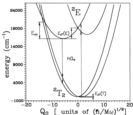
FIG. 4. Configuration-coordinate diagram for \text{Ti}^{3+}:\text{sapphire} , cross-section direction. Intersystem crossing is not discontinuous, since the diagram has been calculated in the diabatic limit.
