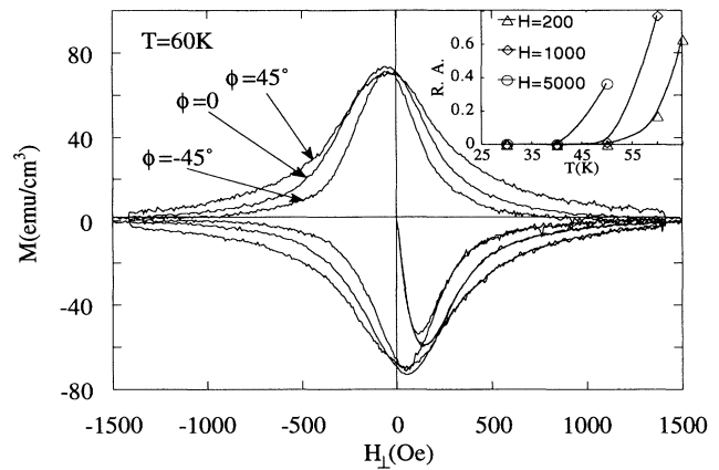
FIG. 2. Magnetization curves of IR45 at T = 60 K, where the field is at angles \phi = 0^\circ and \pm 45^\circ with respect to the c direction. Note that M = m / \cos\phi , where m is the measured magnetization, and H_1 = H \cos\phi . Inset: the temperature dependence of the relative anisotropy (RA) in IR45 at various fields.
