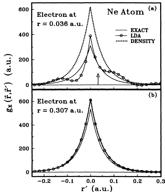
FIG. 1. Pair-correlation density g_x(\mathbf{r}, \mathbf{r}') for the neon atom as determined within the local-density approximation for exchange (LDAX) and Hartree-Fock theory (Exact). The cross section in the electron-nucleus ( \theta' = 0 ) plane is plotted as a function of the distance r' from the nucleus for electron positions at (a) r = 0.036 a.u. and (b) r = 0.307 a.u. The Hartree-Fock theory electronic density is also plotted.
