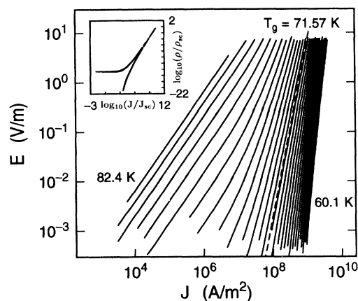
FIG. 1. Log-log plot of some selected I - V isotherms for H = 5 T and \theta = 30^\circ . The field is directed perpendicular to the current. The I - V curves differ by a temperature interval of 0.8 K. The inset shows the scaling collapse of these data for T_g = 71.57 K, z = 5.85 , and \nu = 1.70 . In the scaling procedure J is scaled by J_{sc} \propto T|T - T_g|^{2\nu} , and \rho by \rho_{sc} \propto |T - T_g|^{\nu(z-1)} .
