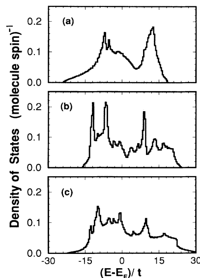
FIG. 3. Conduction-band densities of states (for fixed spin) obtained for (a) the A_4 structure with the four molecules in the same orientations; (b) the A_3B structure, with one of the molecules in the conventional cell flipped to the B orientation; (c) the A_2B_2 structure with two molecules flipped to the B orientation. To obtain three electrons per C_{60} molecule E_F is fixed to be -0.75t for A_4 , -1.90t for A_3B , and -2.05t for A_2B_2 .
