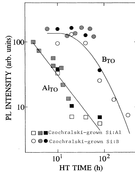
FIG. 4. Annealing-time dependence of the TO replica intensity of acceptor-bound-exciton recombination for material doped with boron ( \circ ) and aluminum ( \square ). For both kinds of materials the results for three different samples—open, cross-hatched, and closed symbols—are given. The curves through the points guide the eye.
