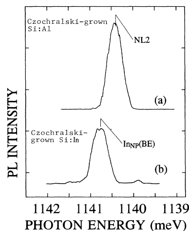
FIG. 9. Comparison of the PL-Si-NL2 line with indium-bound exciton emission, \text{In}_{\text{NP}}(\text{BE}) ; PL spectra were recorded for (a) aluminum-doped Czochralski-grown silicon substrates annealed for 17 h at 470^\circ\text{C} , and (b) indium-doped Czochralski-grown silicon substrates.
