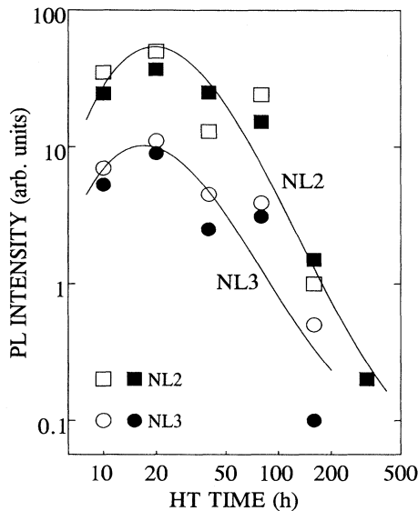
FIG. 7. Generation kinetics during heat treatment at 470 °C of the PL-Si:NL2 ( \square ) and PL-Si-NL3 ( \circ ) lines. The measurements were performed on two samples—open and closed symbols, taken from the same ingot of aluminum-doped Czochralski-grown silicon. The curves through the points serve as a guide to the eye.
