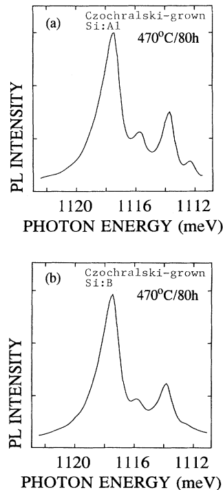
FIG. 3. O_j photoluminescence spectra as recorded for (a) Cz-Si:Al and (b) Cz-Si:B, both thermally treated for 80 h at 470°C.
