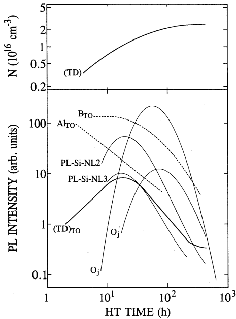
FIG. 8. Combined dependence of all TD-related PL bands investigated in this study on the annealing time (lower part). The intensities of individual PL bands have been scaled to equal laser power. In addition, the TD development kinetics are given as determined on the basis of resistivity measurements on the material used in this study (upper part).
