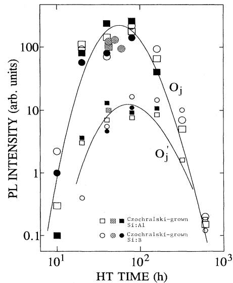
FIG. 2. Development kinetics for the O_j and O'_j bands for Czochralski-grown silicon substrates doped with boron ( \circ ) and aluminum ( \square ). For every dopant the results as obtained for three different samples are presented. The curves through the points serve as a guide to the eye.
