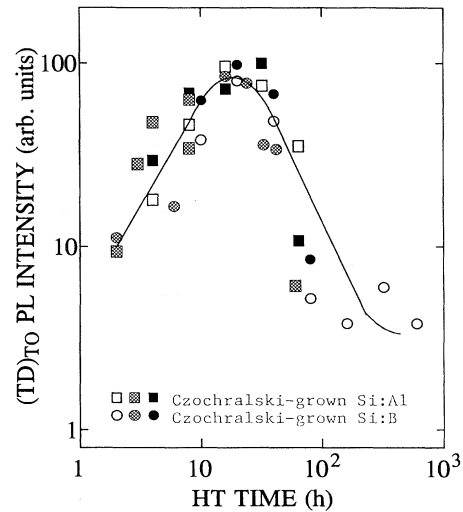
FIG. 1. Intensity of the TO replica of the TD 0 -bound-exciton line as a function of 470^\circ\text{C} annealing time for Czochralski-grown silicon substrates doped with boron ( \circ ) and aluminum ( \square ). For both materials the results as obtained for three different samples of the same ingot are presented, as indicated by open, cross-hatched, and closed symbols. The line is drawn as a guide to the eye.
