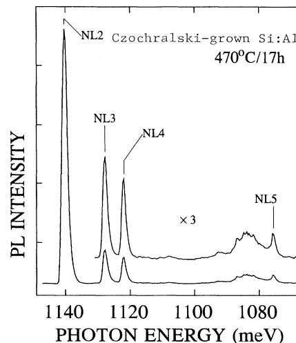
FIG. 6. Photoluminescence spectrum of a Cz-Si:Al sample after an anneal for 17 h at 470°C. The PL-Si- NL_j lines ( j = 2, 3, 4, or 5 ) are indicated.
