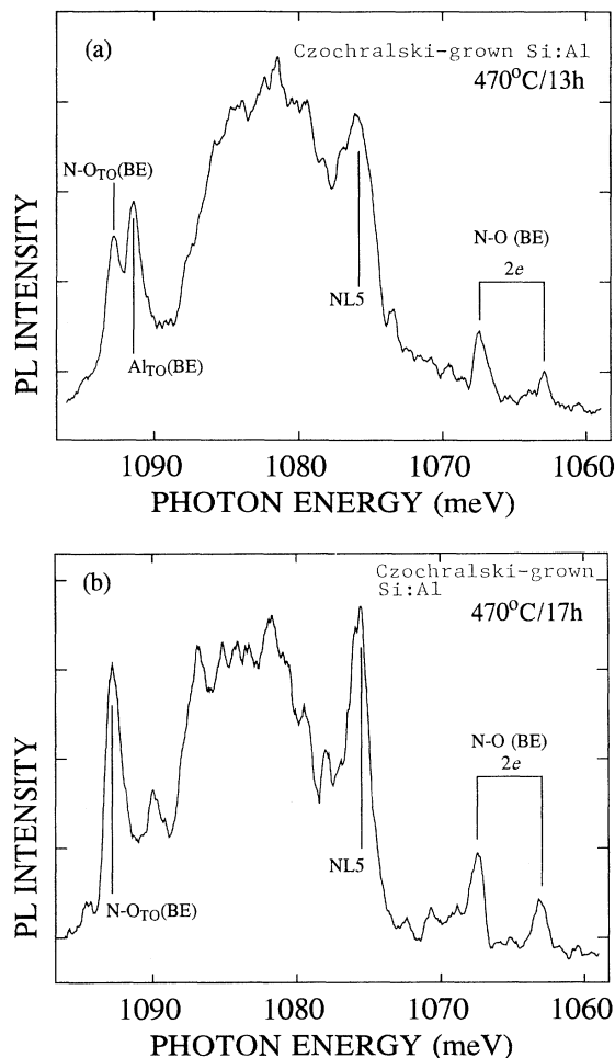
FIG. 5. Photoluminescence from N-O complexes: the PL spectrum as recorded for a Cz-Si:Al sample following a heat treatment at 470°C for (a) 13 h and (b) 17 h. The TO replica as well as two-electron ( 2e ) transitions are indicated.
