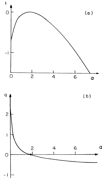
FIG. 2. Multifractal functions based on the approximant of Eq. (5.2) in two dimensions (after Ref. 12). (a) f(\alpha) . (b) q(\alpha) .
