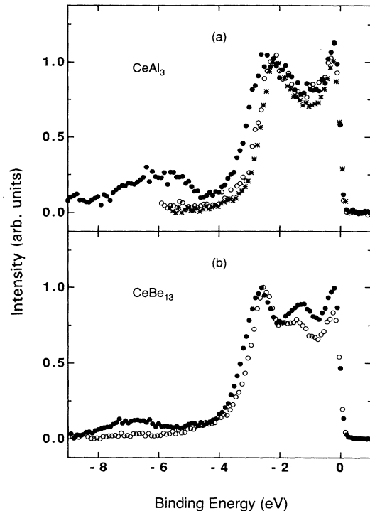
FIG. 1. (a) Valence-band PES of \text{CeAl}_3 at h\nu=120 eV taken with increasing time to show the effect of oxidation on the line shape. Fresh cleave, T=20 K, crosses; 4 h after cleave, T=20 K, open circles; 6 h after cleave, T=300 K, solid circles. (b) Spectra for \text{CeBe}_{13} at h\nu=120 eV and 300 K. Freshly cleaved sample, open circles; 2 h after cleave, solid circles.
