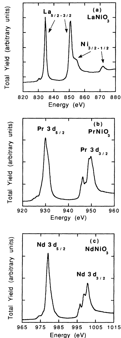
FIG. 6. Room-temperature 3d_{5/2-3/2} edges of (a) La in LaNiO 3 , (b) Pr in PrNiO 3 , and (c) Nd in NdNiO 3 .
