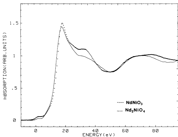
FIG. 8. Room-temperature Ni 1s edges of \text{NdNiO}_3 and \text{Nd}_2\text{NiO}_4 .
