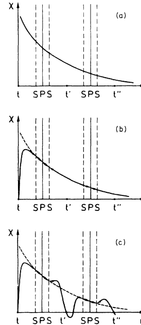
FIG. 1. Construction of the muffin-tin orbital: (a) the original envelope function, (b) substitution of the divergent part in the MT sphere at the origin by the linear combination of numerical radial functions and regular Bessel's function as well as substitution in all other (except the origin) polyhedra of the tail by its one-center expansion in Bessel's functions (illustrated by arrows), (c) substitution of Bessel's functions in all MT spheres by numerical radial functions. Vertical lines show the boundaries s of the MT spheres and the polyhedra.
