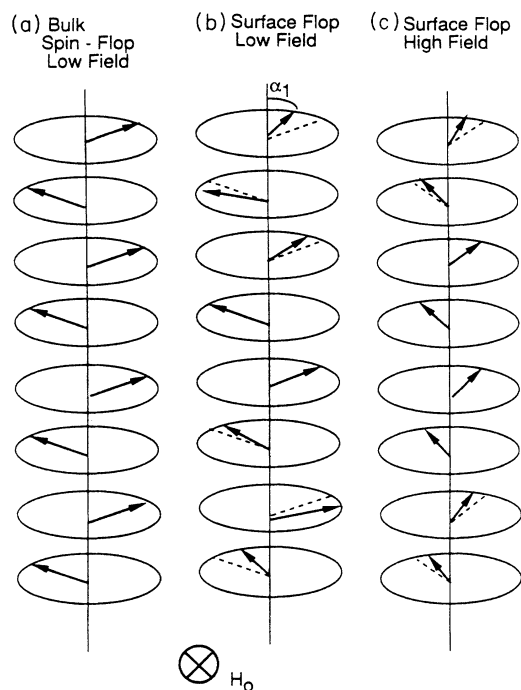
FIG. 1. Examples of possible configurations for a multilayer composed of antiferromagnetically coupled ferromagnetic thin films. The magnetization of each thin film n lies in the plane of the film, is represented by an arrow, and makes an angle \alpha_n with the external field H_0 . In (a) the "bulk" state is shown where \alpha_n is the same for all films. (b) and (c) show configurations for a finite multilayer, with the upper part of the diagram being the top surface of the multilayer and the lower part shows the bottom surface of the multilayer. The dashed lines in (b) and (c) show the "bulk" configuration for these cases. Note that for (b) the outermost spins are turned into the direction of the field, but that the next layer has the spins turned away from the field when compared with the bulk configuration.
