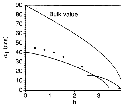
FIG. 8. First angle \alpha_1 is shown as a function of applied field. The solid lines are the results from the variational calculations and the dots are the results from the numerical calculation. The agreement between the two methods improves with increasing field as the magnitude of \alpha_1 decreases.
