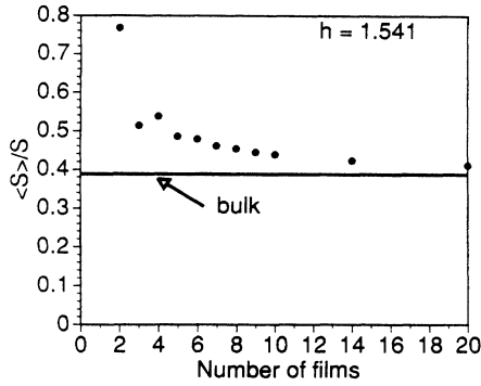
FIG. 4. Average magnetization for a multilayer as a function of the total number of layers. The applied field is h = 1.541 . The nonuniform twist states exist because of the reduced symmetry of the end films. As a consequence, the net deviation from the bulk state increases with decreasing number of layers, which leads to an increasing magnetization. Note the difference between even numbers of films and odd numbers of films.
