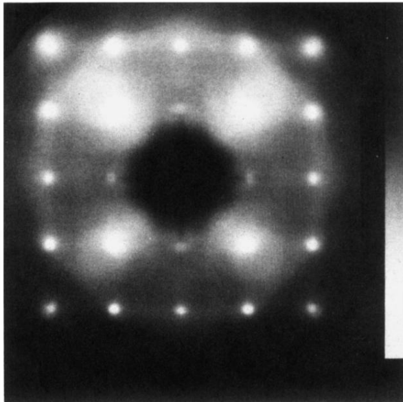
FIG. 1. Experimental LEED pattern for O/Ni(100)—disordered—at approximately 15/100 coverage, T=80 K, and E=650 eV.
