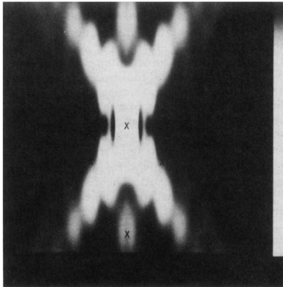
FIG. 4. Atomic-resolution holographic image for E = 650 eV. A plane perpendicular to the surface passing through the adsorbed oxygen and two neighboring nickel atoms. The atomic positions are represented by crosses.
