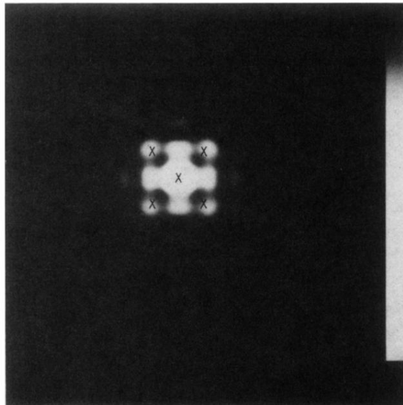
FIG. 2. Atomic-resolution holographic image for E=650 eV. A plane parallel to the surface passing through z=-0.9 . The atomic positions are represented by crosses.
