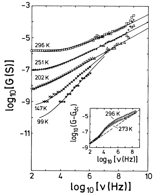
FIG. 2. Frequency dependence of the conductivity at different temperatures. \log_{10}G is plotted vs \log_{10}\nu : 296 K ( \square ); 251 K (+); 202 K ( \triangle ); 147 K ( \times ); and 99 K (*). The solid lines were calculated as described in the text. The inset shows the data at 296 K and at 273 K after subtraction of the dc conductivity. The dashed line is an estimate of the frequency dependence of the ac conduction.
