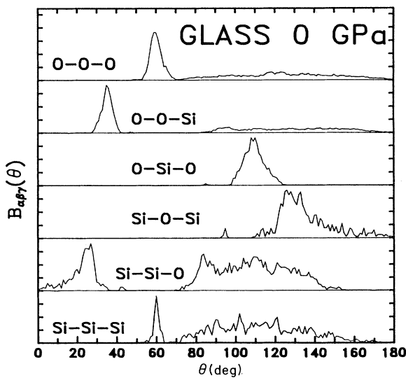
FIG. 8. Angle distributions B_{\alpha\beta\gamma}(\theta) from the Monte Carlo simulations at zero pressure. All distributions are scaled to the same (arbitrary) maximum height.
