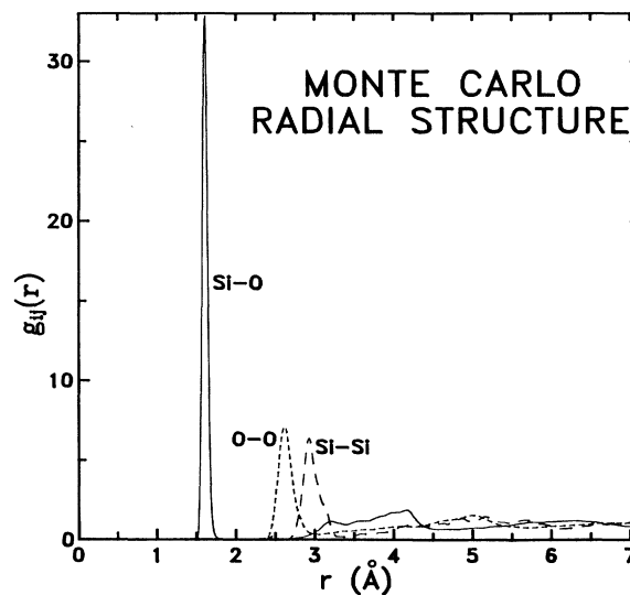
FIG. 3. Component radial distribution functions g_{\alpha\beta}(r) (4) at zero pressure from the Monte Carlo simulations.
