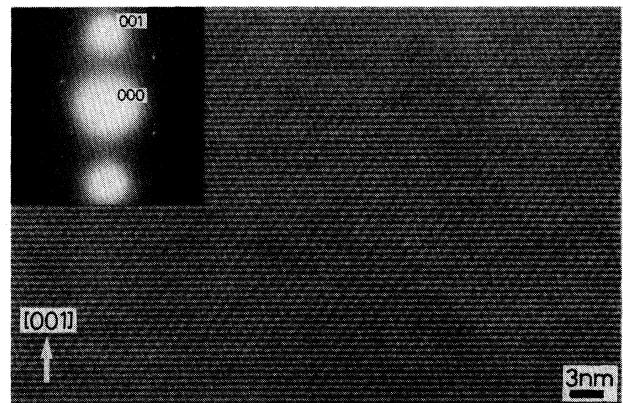
FIG. 20. High-resolution image of the NC phase at 301 K on warming and the corresponding diffraction pattern. The direction of the incident beam is chosen so as to excite a pair of primary spots around 000.
