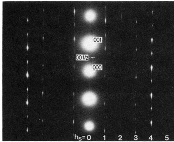
FIG. 14. [140] diffraction pattern of the C phase. The rows of h_s ( =0,1,2,3,4,5 ) mean that of h_s \mathbf{q}_{C1}^e , i.e., indices with subscript of s , have the base vectors \mathbf{q}_{C1}^e and \mathbf{q}_{C2}^e in the basal plane, and \zeta is a coordinate in the unit of |\mathbf{c}^*| .
