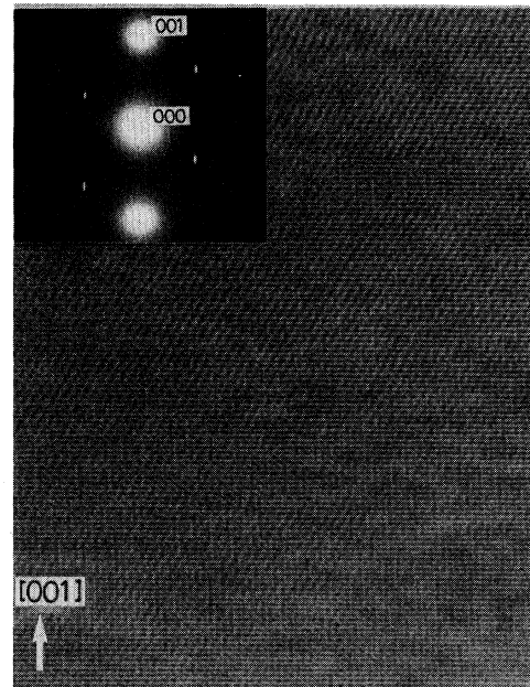
FIG. 19. High-resolution image and diffraction pattern of the T phase at 226 K. The direction of the incident beam is chosen so as to excite a pair of primary spots around 000.
