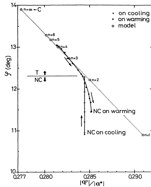
FIG. 24. Relation between |\mathbf{q}^P|/|\mathbf{a}^*| and \phi . Open circles indicate the change on cooling from the IC phase, while solid circles indicate the change on warming. The dotted line indicates the relation |\mathbf{q}^P|/|\mathbf{a}^*| - \phi calculated from the idealized model of the discommensurate network.
