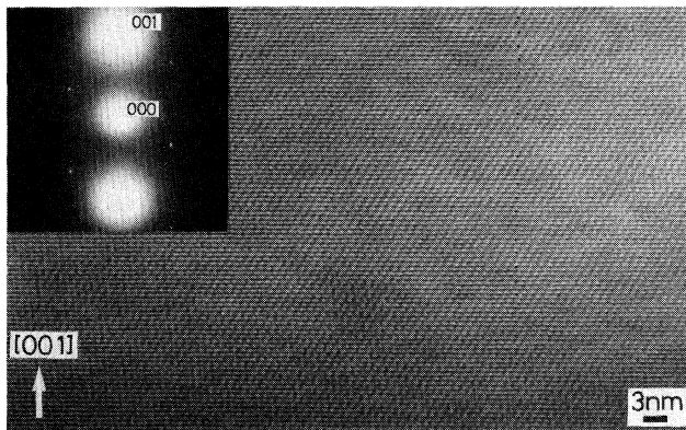
FIG. 10. High-resolution image of the NC phase on cooling at room temperature. The observed direction is perpendicular to the c axis, exciting a pair of primary spots.
