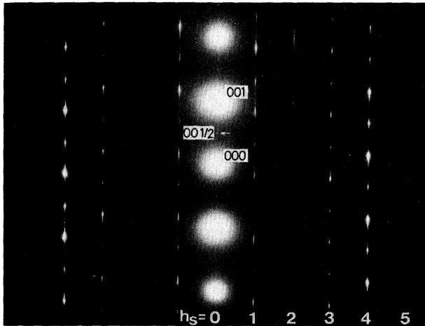
FIG. 14. [140] diffraction pattern of the C phase. The rows of h_s , ( =0,1,2,3,4,5 ) mean that of h_s \mathbf{q}_{C_1}^s , i.e., indices with subscript of s , have the base vectors \mathbf{q}_{C_1}^s and \mathbf{q}_{C_2}^s in the basal plane, and \zeta is a coordinate in the unit of |\mathbf{c}^*| .
