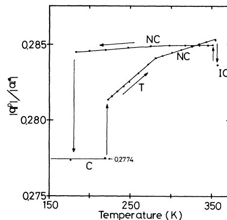
FIG. 3. Temperature dependence of |q^p|/|a^*| . Note the change of slope at \sim 280 K between the T phase and the NC phase on warming.
