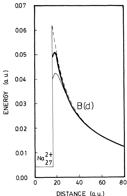
FIG. 4. Calculated capture barrier for the reaction \text{Na}_{26}^{+} + \text{Na}^{+} \rightarrow \text{Na}_{27}^{2+} . The meaning of the different lines and symbols is as in Fig. 3.
