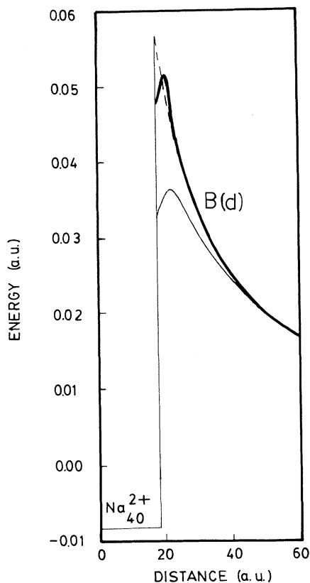
FIG. 5. Calculated capture barrier for the reaction \text{Na}_{39}^{+} + \text{Na}^{+} \rightarrow \text{Na}_{40}^{2+} . The meaning of the different lines and symbols is as in Fig. 3.
