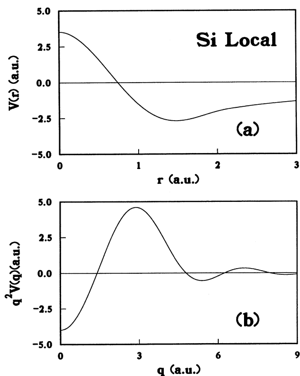
FIG. 1. The local silicon ionic pseudopotential (a) and its Fourier transform (b) obtained from the variational minimization procedure given in Sec. III.
