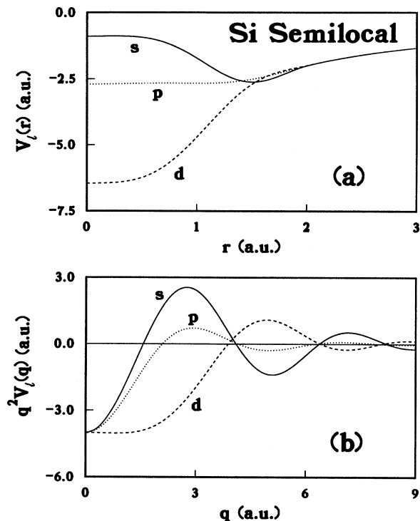
FIG. 3. The semilocal pseudopotential (a) and its Fourier transform (b) used in Sec. V. The pseudopotential was obtained using the method of Ref. 6.
