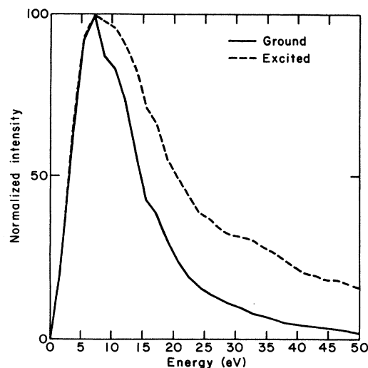
FIG. 2. Experimental angle-integrated energy distributions of the ground-state (solid curve) and excited-state (dashed curve) Rh atoms ejected from ion-bombarded Rh{100} surface in the (010) plane. The distributions are normalized to the peak intensity.
