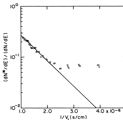
FIG. 4. Ratio of the excited-state distribution dN^*/dE , to the ground-state distribution dN/dE , vs the reciprocal of the normal component of the emission velocity ( v ) for atoms with \theta < 10^\circ . The straight line indicates the best fit to the high-velocity part of the data points.
