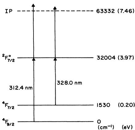
FIG. 1. Schematic energy-level diagram of a rhodium atom illustrating the MPRI schemes used to ionize Rh in the {}^4F_{7/2} excited state and in the {}^4F_{9/2} ground state. IP represents the first ionization potential of Rh atom.
