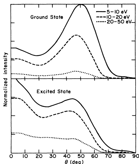
FIG. 3. Measured angular distributions of Rh atoms ejected from Rh{100} surface in the (010) plane. The top curves correspond to the ground-state distributions and the bottom plots to the excited-state distributions for 5–10 eV (solid), 10–20 eV (dashed), and 20–50 eV (dotted) energy ranges, respectively.
