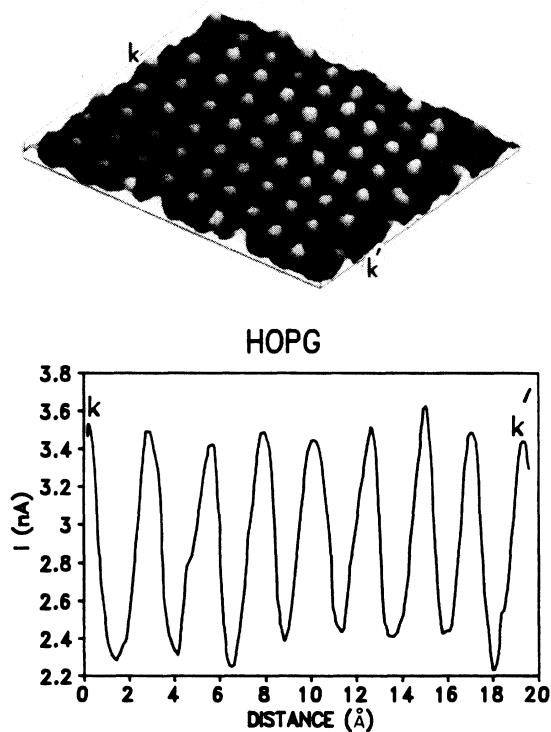
FIG. 2. A 20.75 \times 20.75 -Å 2 atomic-resolution STM image, taken in the current-imaging mode, of the surface of HOPG showing trigonal symmetry. Below is a cross section detailing the atomic separation and the corrugation amplitude. The cross section is taken along a line that connects points k and k' . The atomic separation is 2.45 Å.
