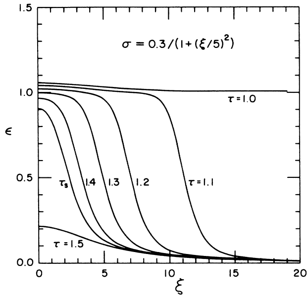
FIG. 4. Strain profiles for different temperatures under the stress field \sigma = \sigma_0 / [1 + (\xi/\xi_0)^2] with \sigma_0 = 0.3 , \xi_0 = 5 . Here \tau_s = 1.4524 is the local martensite formation temperature. For \tau > \tau_s there is only pretransformed distortion of the high-temperature phase as shown by the curve \tau = 1.5 .
