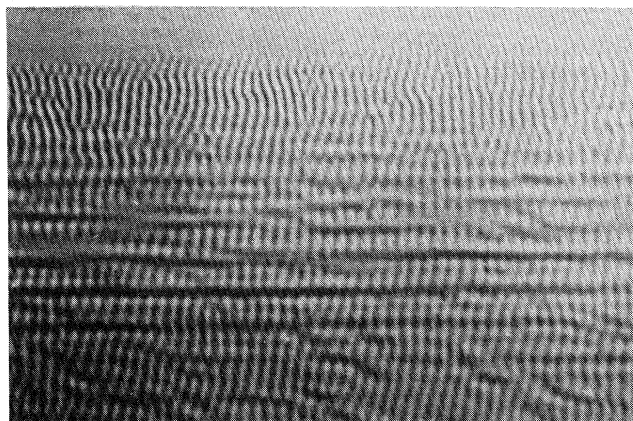
FIG. 2. Germanium sample, S -polarized light incident at 70^\circ , magnification XM 1250. The variation of spacing vertically along the picture is believed to be associated with a varying dielectric constant due to a temperature gradient. Also note large near horizontal b -type fringes of spacing \approx 8 \mu\text{m} .
