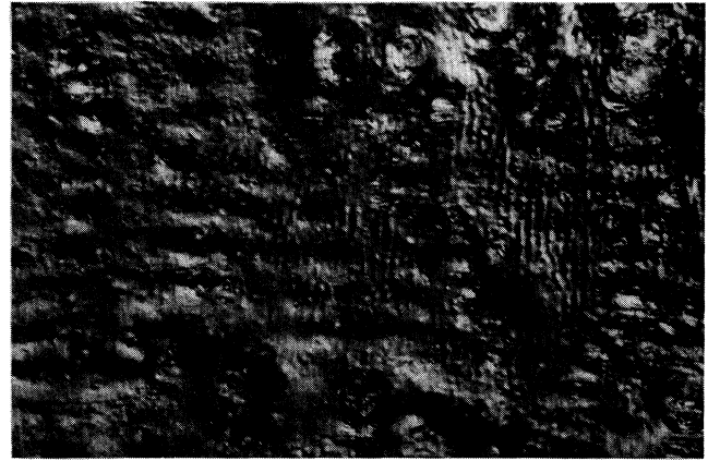
FIG. 8. ALIPSS on Al sample P -polarized light incident 60^\circ , magnification XM 1250. Observe the p^{*-} (horizontal with large spacing) and c^* (vertical and of smaller spacing) ripples. Ripple morphology is similar to normal LIPSS but the spacing is about eight times too big.
