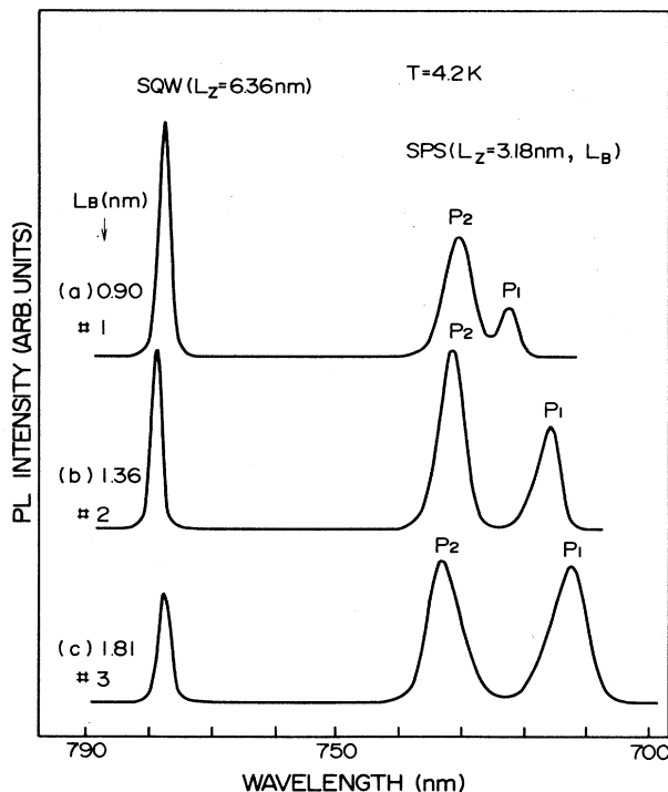
FIG. 2. Photoluminescence spectra of SQW-embedded SPS samples at 4.2 K: (a) sample 1, (b) sample 2, and (c) sample 3. The excitation density is about 10^{14} \text{ cm}^{-3} .
