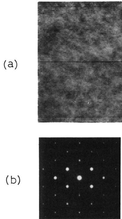
FIG. 1. (a) Cross-sectional image and (b) diffraction pattern by transmission electron microscopy of sample 1, L_z = 6.36 nm GaAs SQW confined by GaAs/AlAs SPS ( L_z = 3.18 nm and L_B = 0.90 nm, 40 periods below and above).
