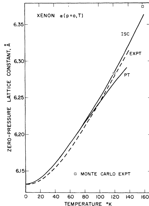
FIG. 2. Zero-pressure lattice constant of solid Xe. ISC and PT were calculated using a (12-6) LJ potential with F_{ISC} and F_{PT} , respectively (see Ref. 5). Experimental data are taken from a compilation in Ref. 19. Monte Carlo results are shown as squares.
