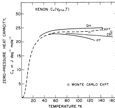
FIG. 4. Zero-pressure C_v for solid Xe. The curves QH, ISC, PT were calculated from F_{QH} , F_{ISC} , and F_{PT} , respectively (see Ref. 5). The Monte Carlo results are shown as squares. Experimental data are from Ref. 19.
